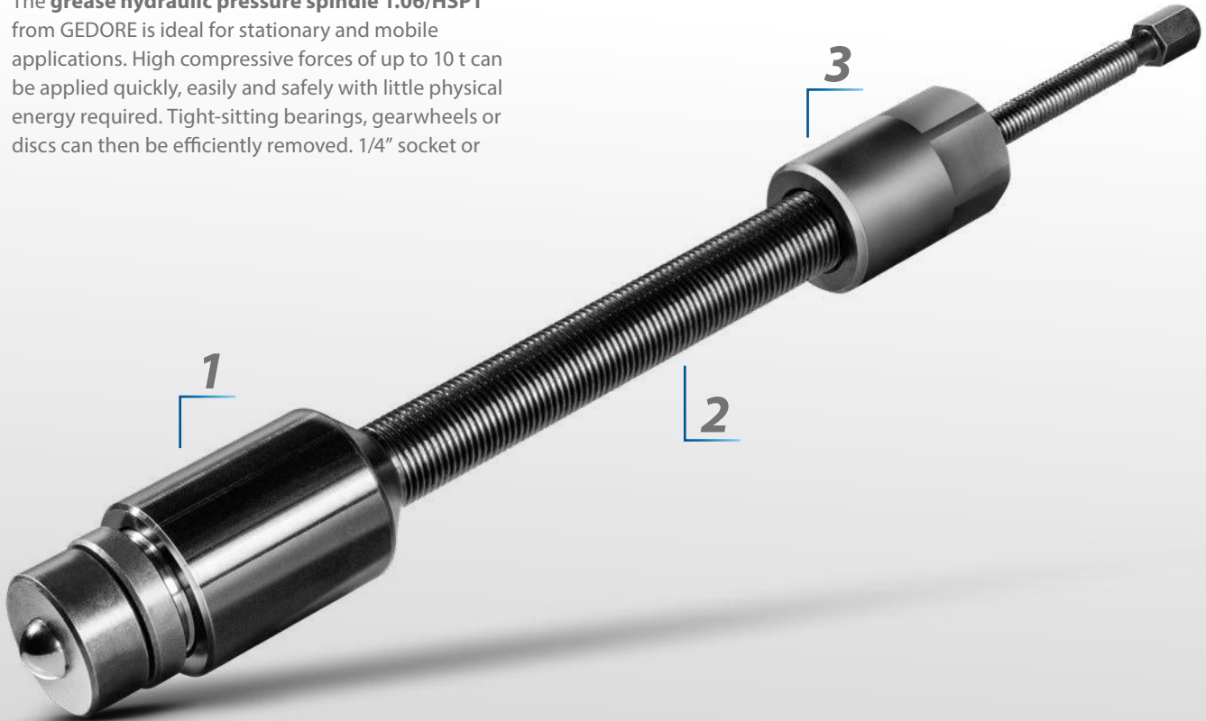
Grease hydraulic pressure spindle – 1.06/HSP1
