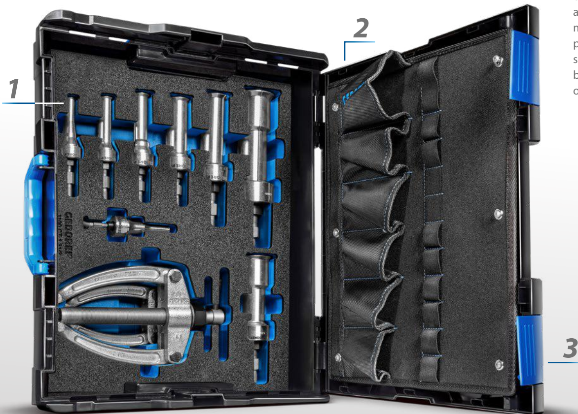
Internal puller set in L-BOXX – 1100-1.31/2
