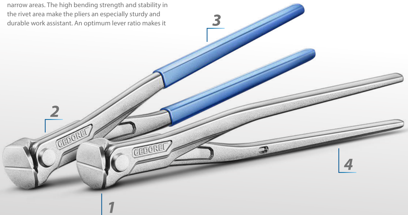
Reinforcing steel pliers – 8380 L
