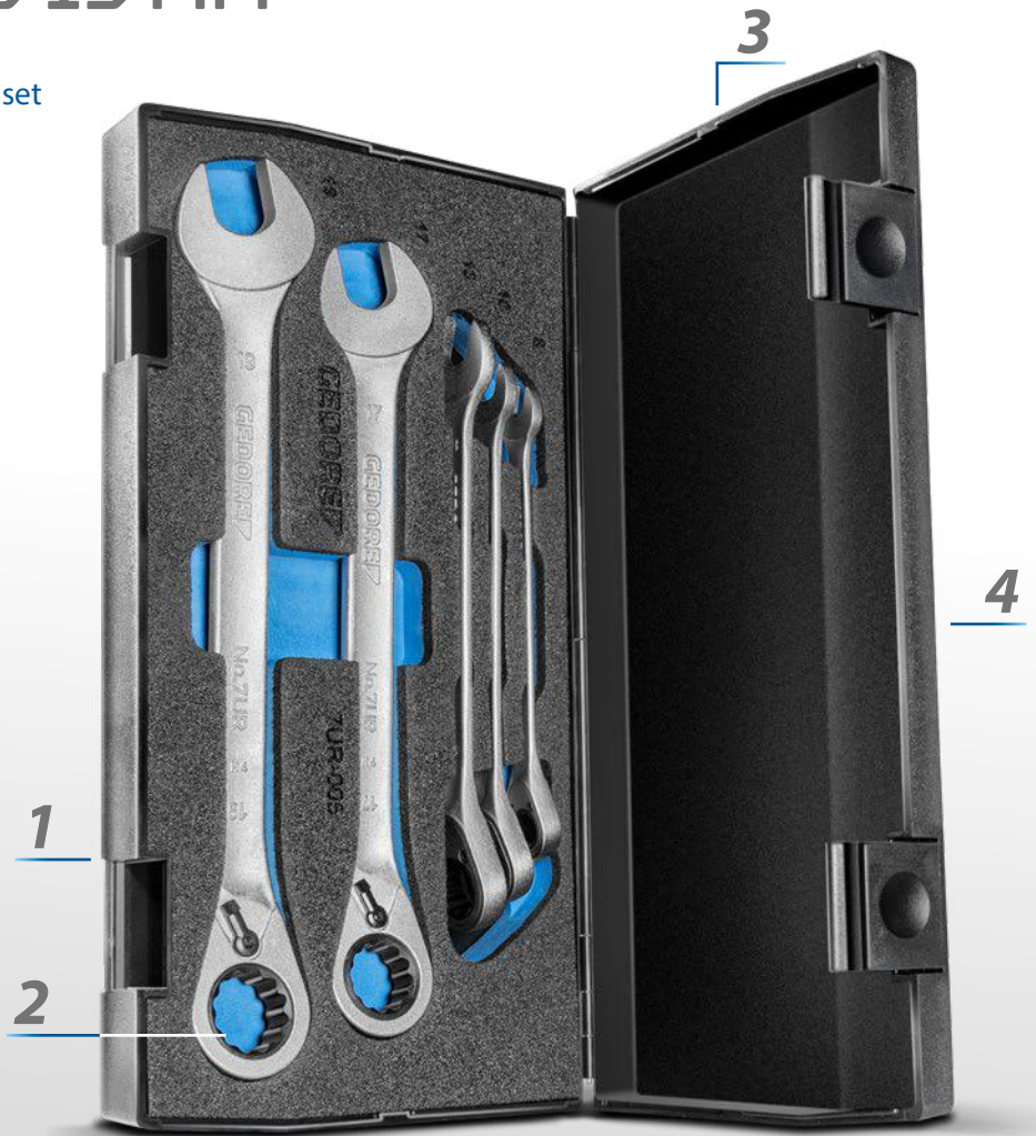
Combination ratchet wrench set, 5-piece – 7 UR-005
